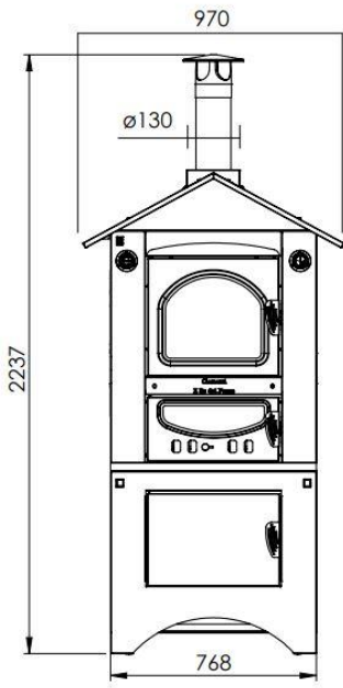
SMART 45x80 cm - 280 kg
